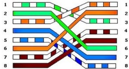
TIA/EIA 568B Crossed Wiring
